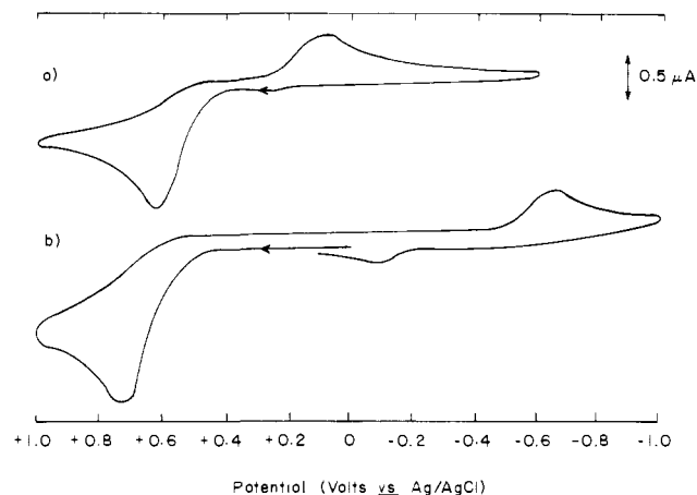
Figure 3. Cyclic voltammograms for 1 mM (C_6Me_6)W(CO)_3 ( 4 ) at platinum disk electrode (0.1 M TEAP, 200 mV/s scan rate). Solvent: (a) CH_3CN ; (b) DMF.
