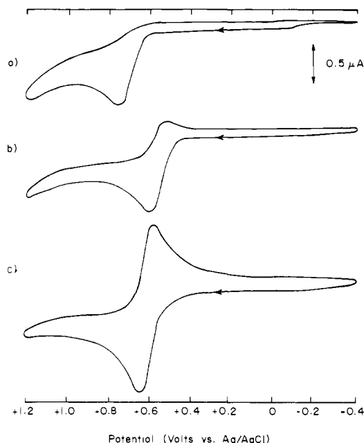
Figure 1. Cyclic voltammograms for 1 mM (arene)chromium tricarbonyl complexes in \text{CH}_3\text{CN} at platinum disk electrode (0.1 M TEAP, 200 mV/s scan rate): (a) (\text{C}_6\text{H}_6)\text{Cr}(\text{CO})_3 ; (b) (\text{C}_6\text{Me}_6)\text{Cr}(\text{CO})_3 ; (c) (\text{C}_6\text{Et}_6)\text{Cr}(\text{CO})_3 .
