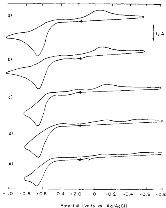
Figure 5. Cyclic voltammograms for 1 mM (C_6Me_6)W(CO)_3 ( 4 ) in CH_3CN at platinum disk electrode (0.1 M TEAP, 200 mV/s scan rate) containing (a) no added ligand, (b) 20 mM P(OPh)_3 , (c) 10 mM PH_3 , (d) 10 mM P(O-n-Bu)_3 , and (e) 10 mM P-n-Bu_3 .
