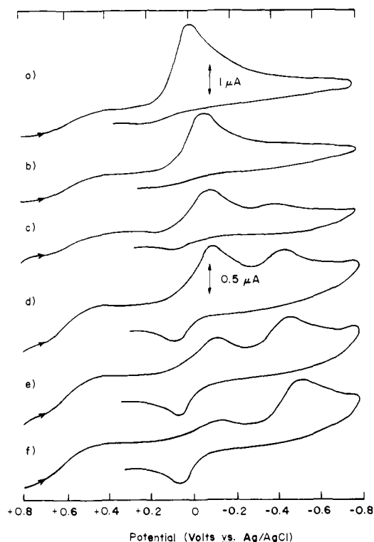
Figure 6. Cyclic voltammograms for 1 mM (C_6Me_6)W(CO)_3 ( 4 ) in CH_3CN at platinum disk electrode (0.1 M TEAP) containing (a) no added PBu_3 , (b) 0.33 mM PBu_3 , (c) 0.67 mM PBu_3 , (d) 1.00 mM PBu_3 , (e) 1.34 mM PBu_3 , and (f) 1.67 mM PBu_3 (held 15 s at +0.8 V and then scanned at 500 mV/s).
