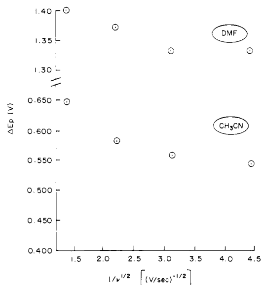
Figure 4. Dependence of peak potential separation ( \Delta E_p ) on scan rate ( \nu ) in cyclic voltammetry of (C_6Me_6)W(CO)_3 ( 4 ) at platinum disk electrode.
